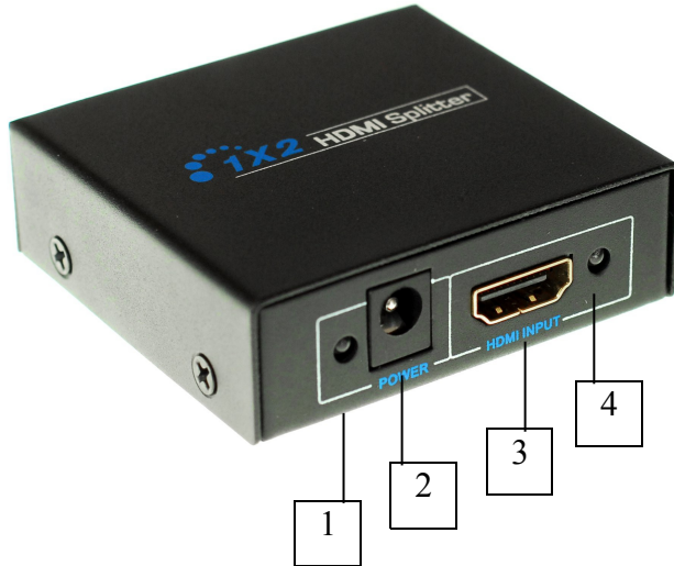
Figure 2: Back Panel
